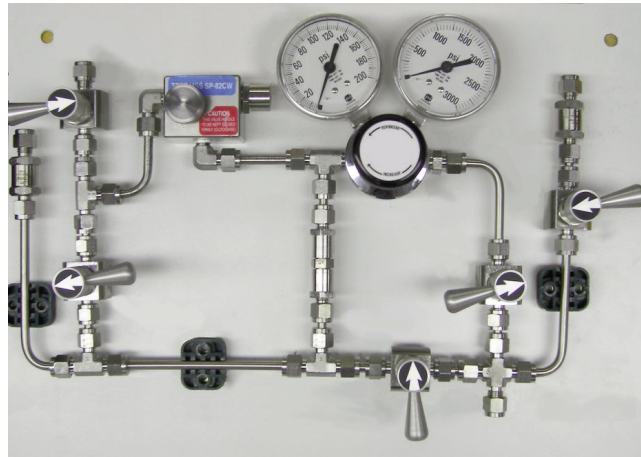
Five-Valve Panel
